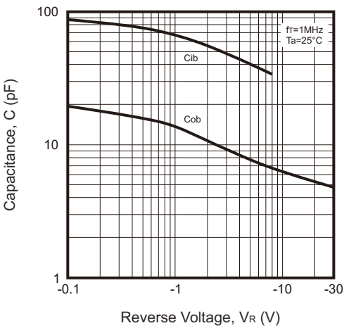
Fig.6 - C_{ob}/C_{ib} \text{ --- } V_{CB}/V_{EB}
